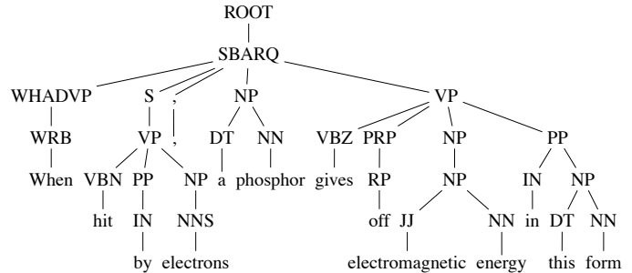
Figure 2: Constituency Tree
