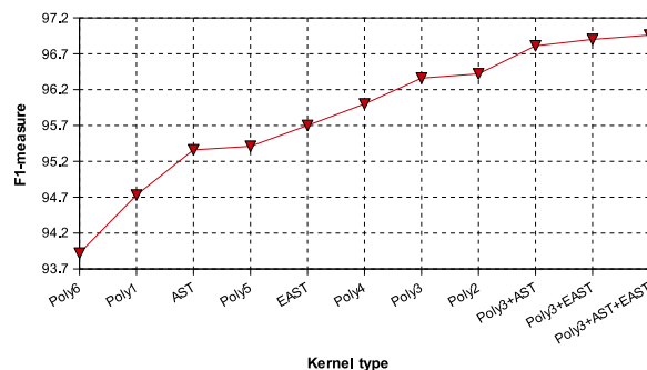
Figure 5: Impact of polynomial kernel, tree kernels and their combinations on boundary detection.
