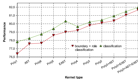
Figure 6: Impact of the polynomial kernel, tree kernels and their combinations on the accuracy in role classification (gold boundaries) and on the F_1 of complete SRL task (boundary + role classification).
