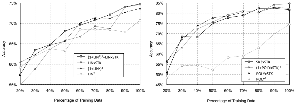
Fig. 4. Learning curves for GEOQUERIES and RESTQUERIES corpora
